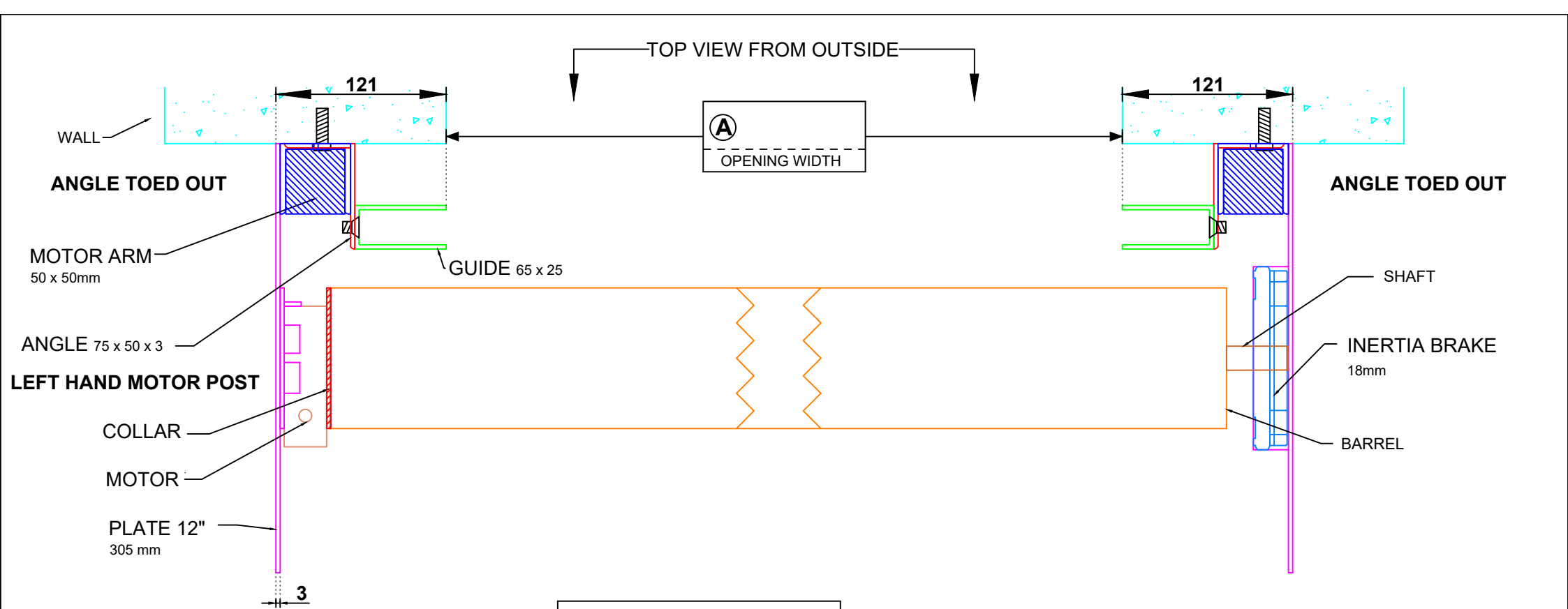
Face fix - Left Hand Motor - Angle Toed Out
