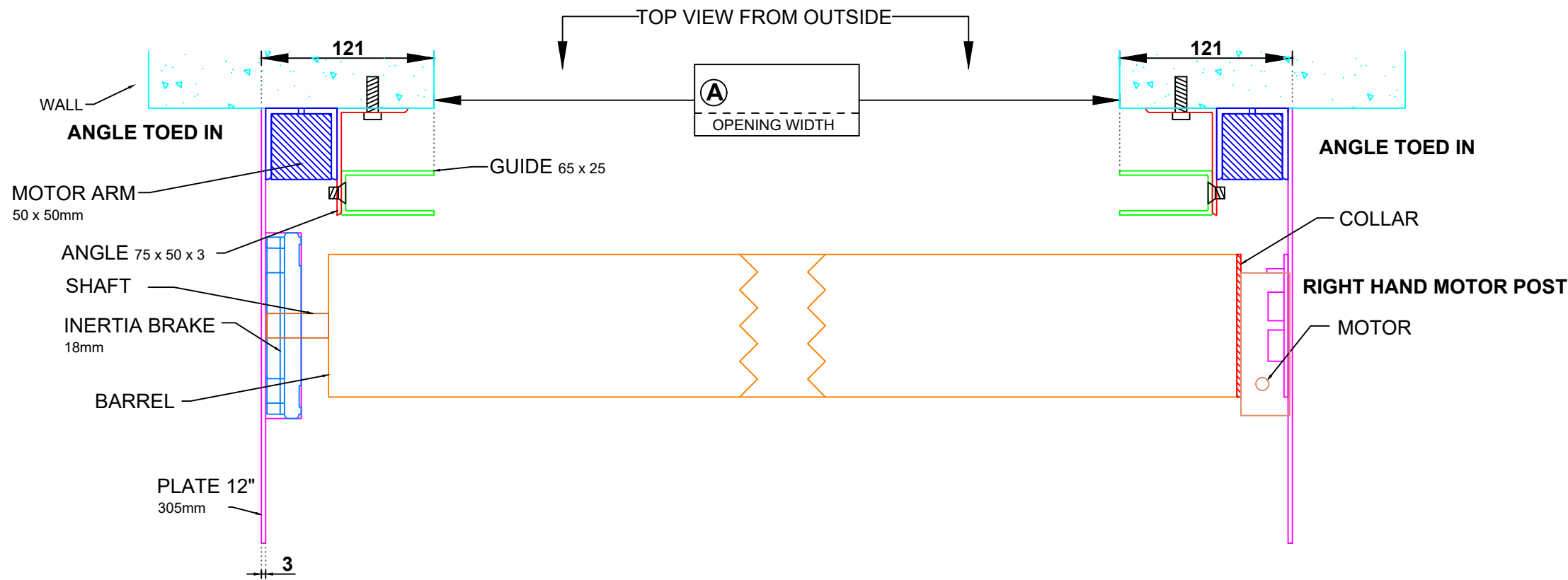
Face fix - Right Hand Motor - Angle Toed In
