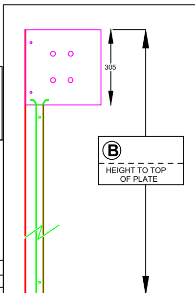
TYPICAL SIDE VIEW
