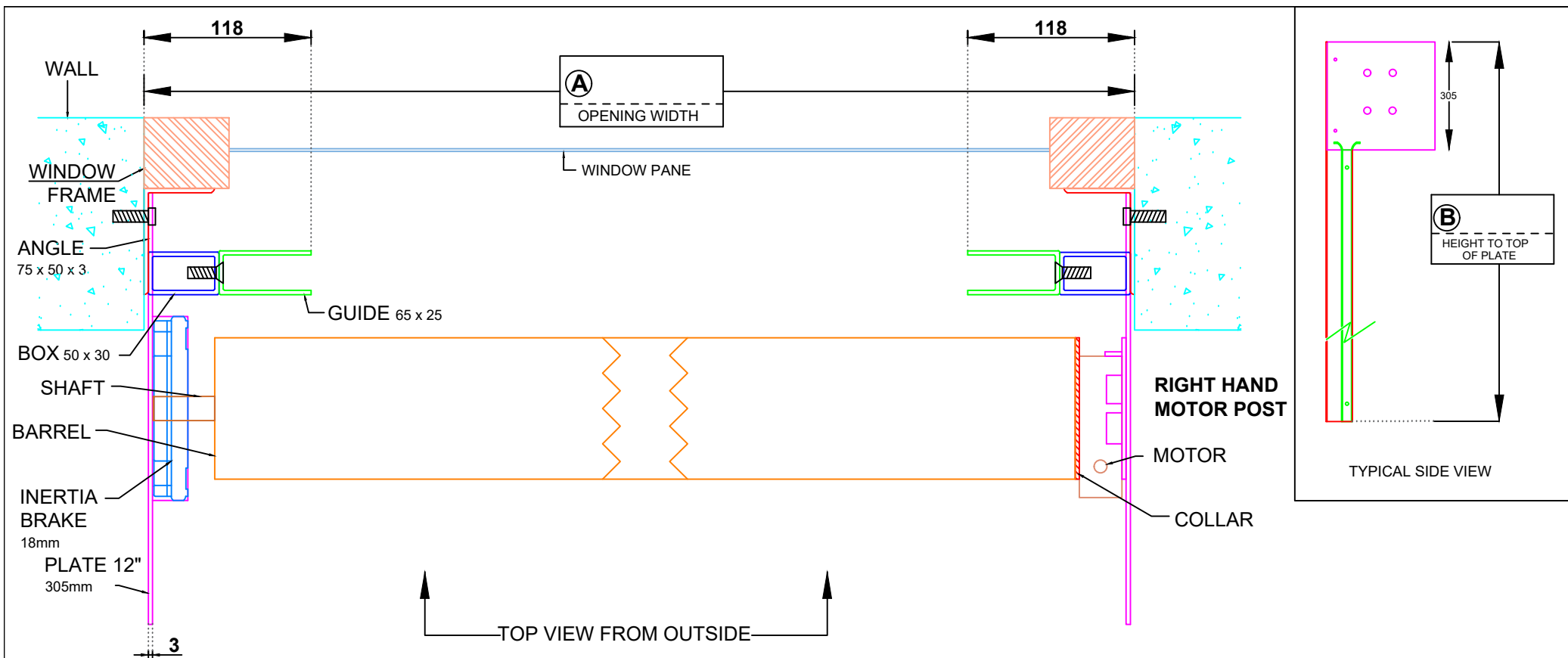
Reveal fix - Right Hand Motor
